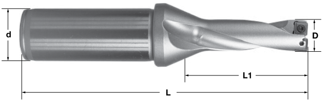
3XD DRILL BODIES - SPMG 050204
