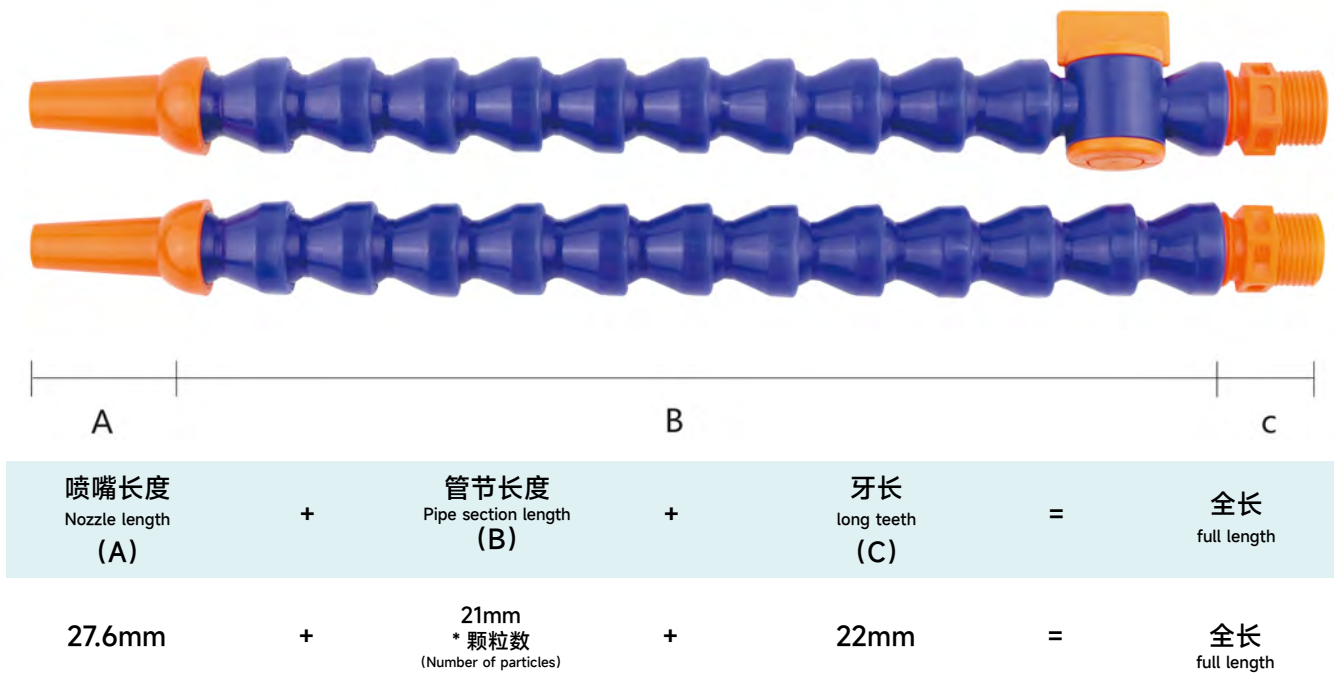
塑料冷却水管配件组配表 ( 可根据要求任意长度管件组装 ) plastic cooling water pipe accessories assembly table(Can be assembled with any length of pipe fittings as required)
