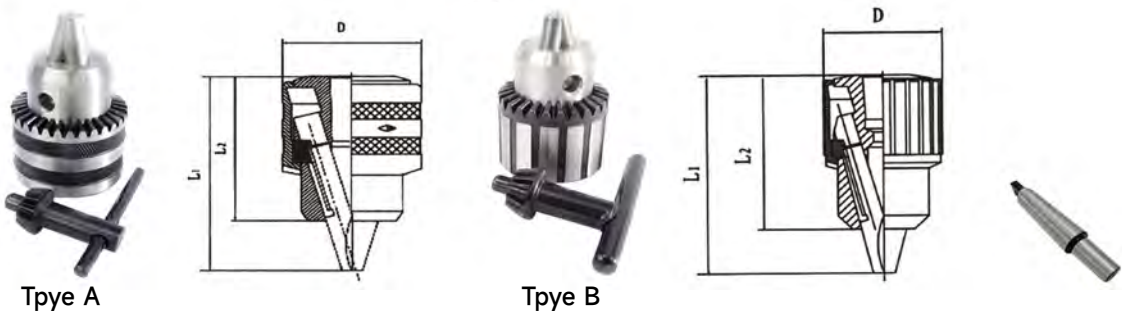
(重型 Heavy Duty) 扳手式锥孔钻夹头 Key-Type Drill Chucks With Taper Fitting
