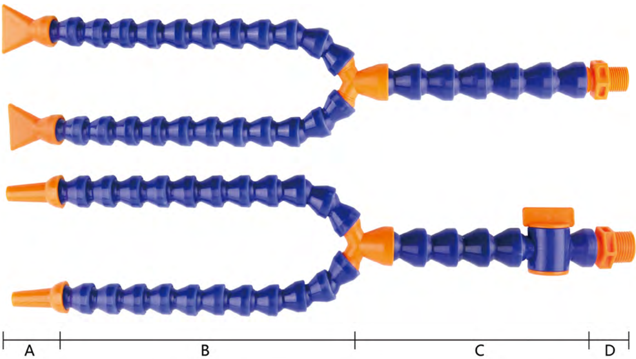
塑料冷却水管配件组配表 ( 可根据要求任意长度管件组装 ) plastic cooling water pipe accessories assembly table(Can be assembled with any length of pipe fittings as required)
